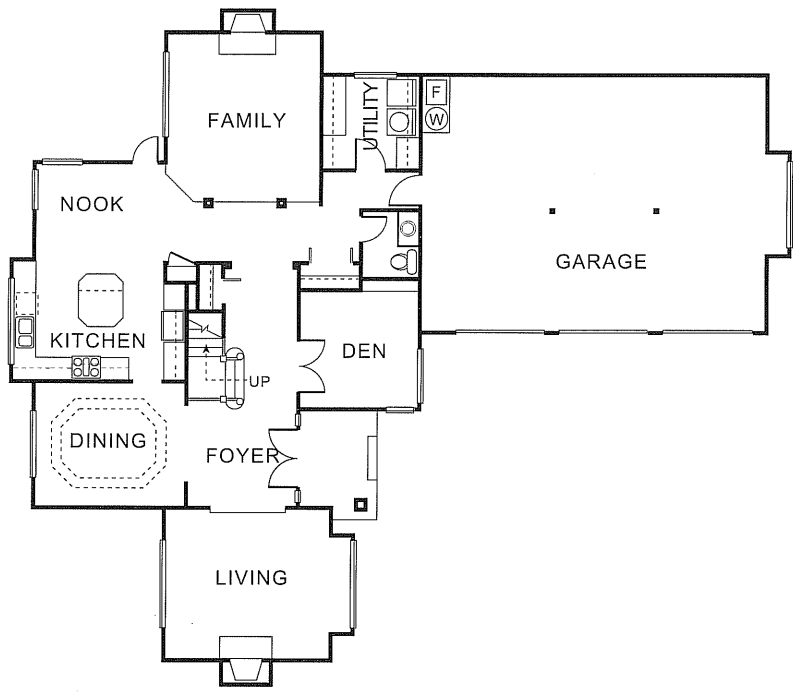
MAIN FLOOR
